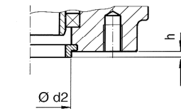
Version Y with spigot
