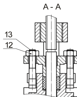
Detail of packing Detail ucpávky
